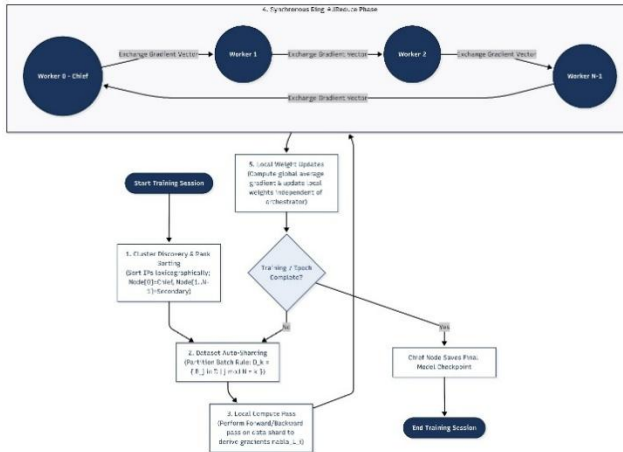
Fig. 6. Distributed machine learning training workflow with Ring-AllReduce
