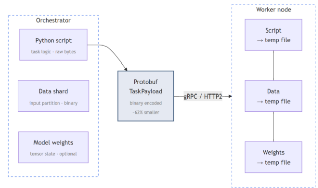
Fig. 4. Data Serialization Pipeline
