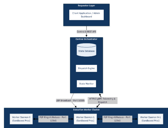
Fig. 1. Three-tier heterogeneous distributed processing architecture
