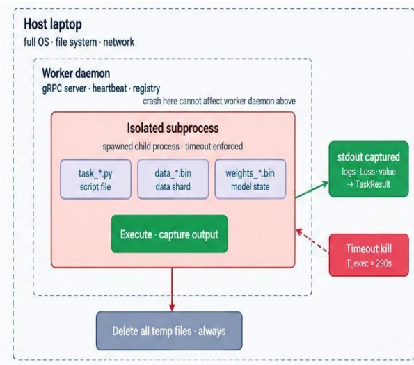
Fig. 5. Execution sandbox architecture
