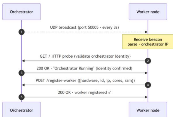
Fig. 2. Discovery and registration sequence
